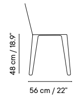
iSi 9135 Chair
