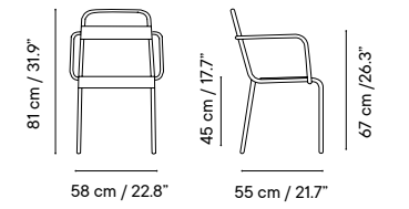
iSi 8056 Armchair
