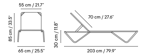
iSi 3024 Sunlounger
