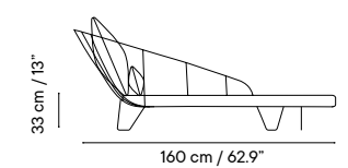
iSi 8123 Daybed
